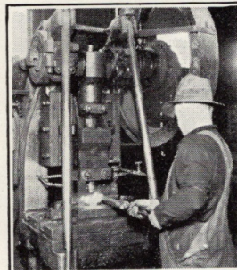
Hot Broaching P & C Box Wrenches with Giant Broaching Press.
