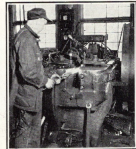
Hot Forging and Hot Broaching P & C Sockets with Heavy Duty Automatic Forging Machine.
