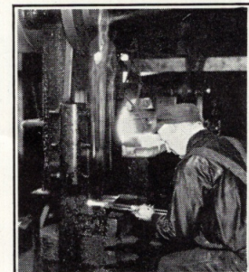
Hand Forging Box Wrenches with Rapid Blow Trip Hammer.
