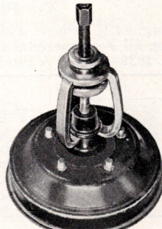
No. 2025-C Jaws Ford 3-Jaw Drum Puller
