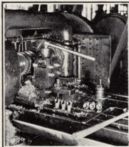
Production Milling Machine for Flex Handles, Universal Sockets, Extensions and other Hand Forged Tools.
