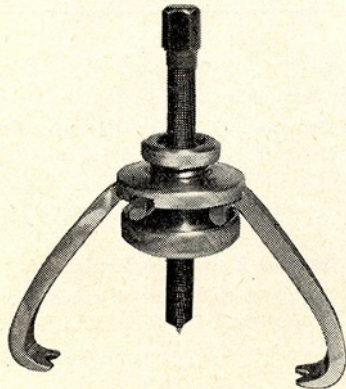
No. 2025-C 2-Jaw Puller For Timing Gears
