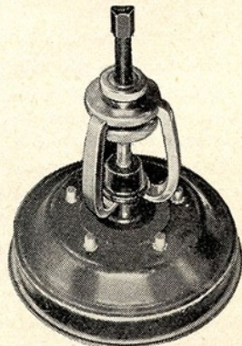
No. 2025-C Jaws Ford 3-Jaw Drum Puller
